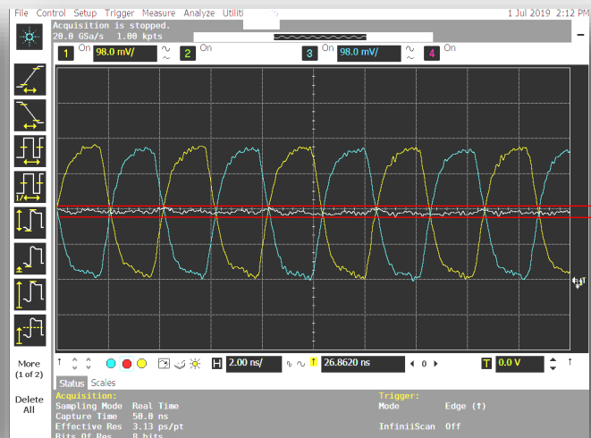
STC-USB2.0R2SのSkew
